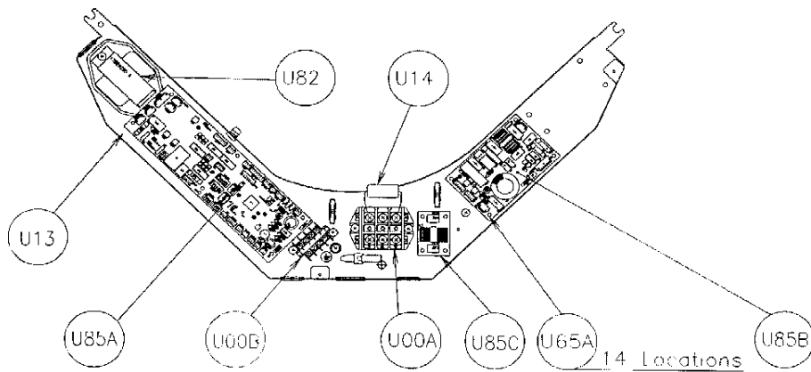
Location of Connectors on PCB for Indoor Units
